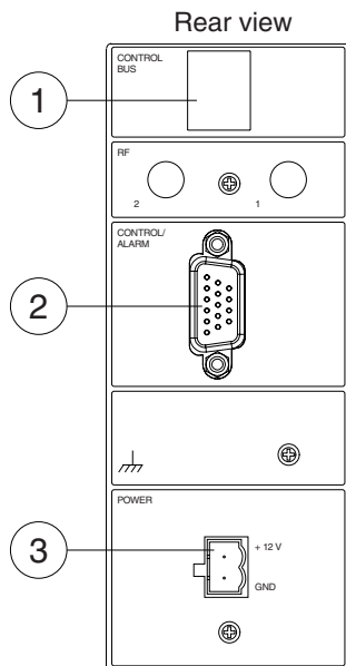
Picture 3. CMA021 Module Adapter 1) RJ-45 female connector, not in use. 2) Control / alarm interface connector (HD15 female). 3) Supply voltage connector.
