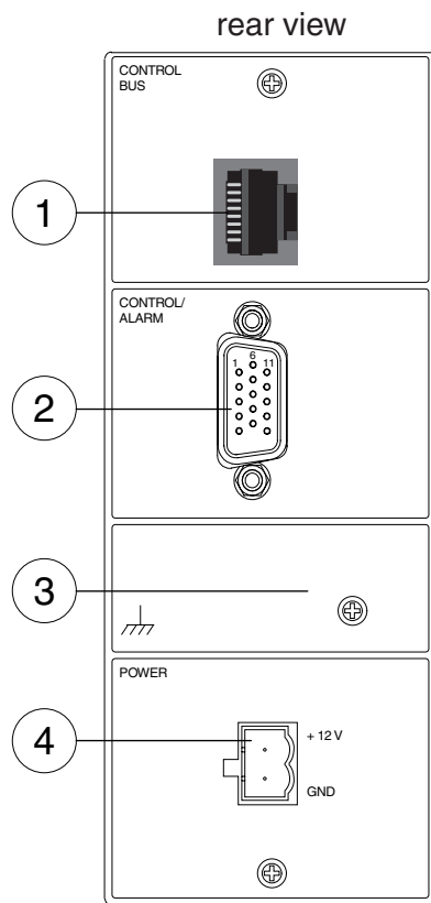
Picture 3. CMA021 Module Adapter 1) Control bus for management systems (RJ-45 female), not in use. 2) Control / alarm interface connector (HD15 female). 3) Grounding connection. 4) Supply voltage connector.
