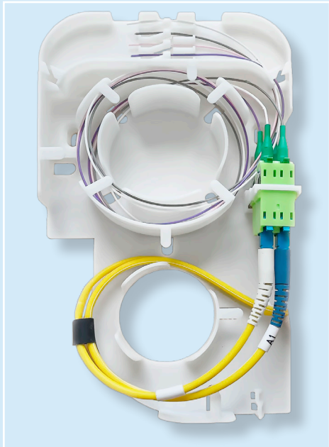
Space for extra fibre/cable routing on both input/drop output sides, with 4 splice locations (heat shrink/crimp), and supports 2 SC adaptor locations.
