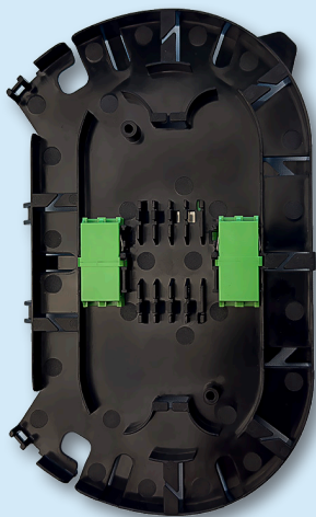
2 populated adapter positions supporting up to 4 connectorised LC drops
