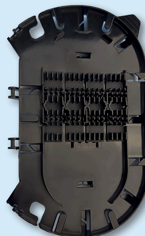
Adapter positions fitted with 3 × 3 fusion-splice click-in inserts, providing capacity for 36 splices
