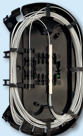
2 adapter positions accept 3 x 3 fusion-splice click-in inserts for up to 18 splices, with 4 dedicated splitter-holder slots alongside
