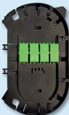
4 populated adapter positions supporting up to 8 connectorised LC drops
